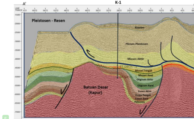
Fig.7 The reinterpretation of seismic data passing through the K-1 well position (modified by [27]).
