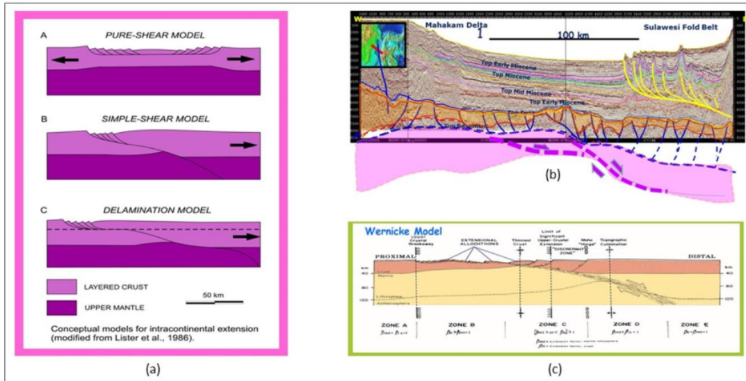
Fig. 5 Several extension models of continental basin formation (a); asymmetric horst-graben geometric association in the Makassar Basin (b); according to [20] model of simple shear kinematics on the formation of basins (c).
