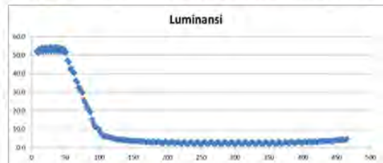
Fig. 14 Simulated luminance curve using double-mounted HPS
