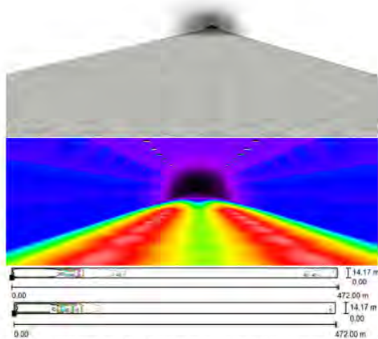
Fig. 12 Simulation results of semicircle tunnel with HPS light using a double mounting
