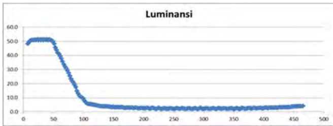
Fig. 13 Simulated luminance curve using single-mounted HPS lamps
