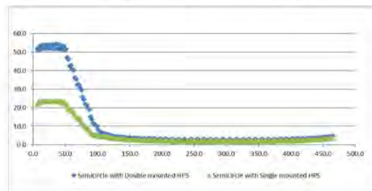
Fig. 16 Luminance Comparison of Double-mounted vs. Single-mounted HPS
