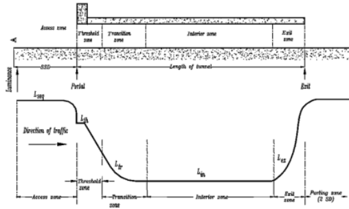
Fig. 4 Five Tunnel Zone [17], [23], [26]
