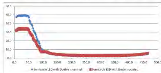
Fig. 15 Luminance Comparison of Double-mounted vs. Single-mounted LED
