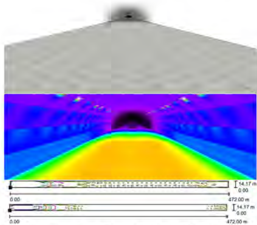
Fig. 8 Simulation results of semicircle tunnel with LED lights with double mounting
